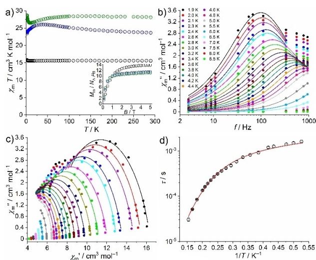
Figure 4. Magnetic dc data of 2–4 : a) \chi_m T vs. temperature T at 0.1 T. Inset: molar magnetization M_m vs. magnetic field B at 2.0 K; experimental data of 2 (green), 3 (blue), and 4 (black open circles), least-squares fit of 4 data using an effective isotropic spin model (solid gray line). (b–d) Magnetic ac data of 2 at a static bias field of 500 Oe: b) Out-of-phase susceptibility \chi_m'' vs. frequency f . c) Cole-Cole plot of \chi_m'' vs. in-phase magnetic susceptibility \chi_m' in the range 1.9–8.5 K (filled circles: data, lines: least-squares fits). d) Arrhenius plot of relaxation times \tau vs. inverse temperature 1/T (the solid red line shows a combined fit considering a direct and a Raman relaxation processes).
